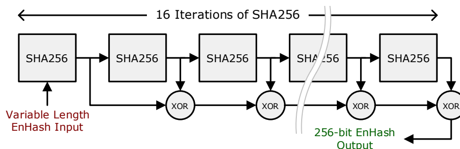
Figure 2: EnHash
