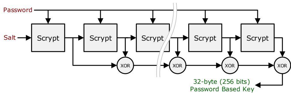
Figure 4: EnScript
