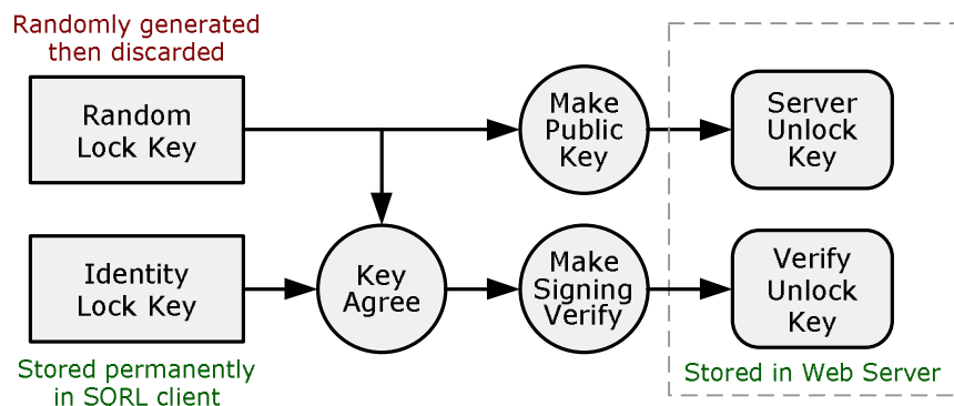
Figure 10: Creating a New Identity Lock Association
